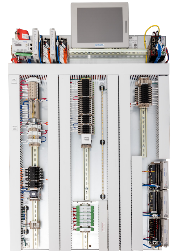
Subplate: installs into existing enclosure
