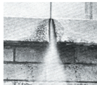
FIGURE 3 Open end of tracing not only loses steam but can also create other maintenance problems such as the corrosion of concrete sill shown here.
